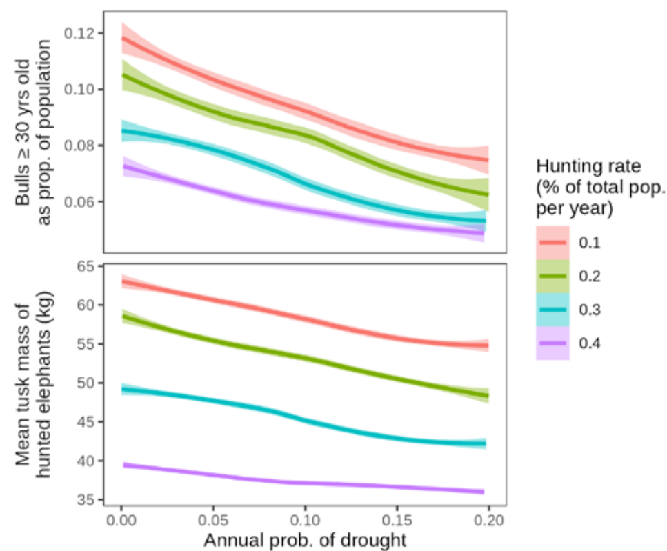
Fig. 5. Effects of drought frequency on hunting outcomes and bull population structure in simulation models. All conventions as in Fig. 3.
